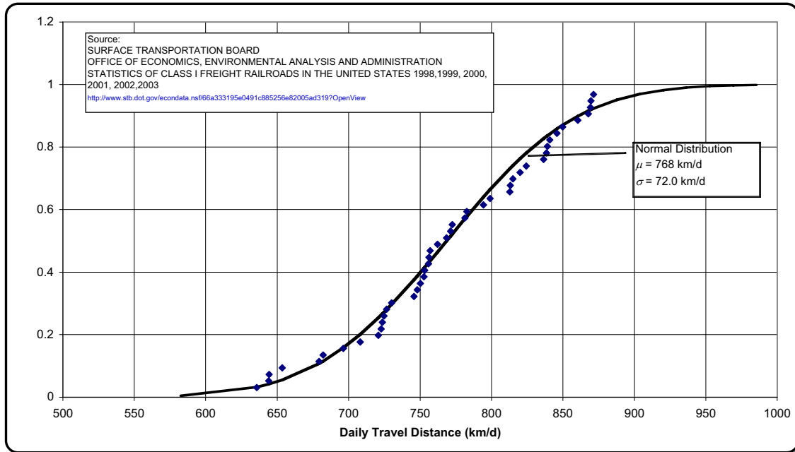
Figure O-32. Estimating train speeds.
