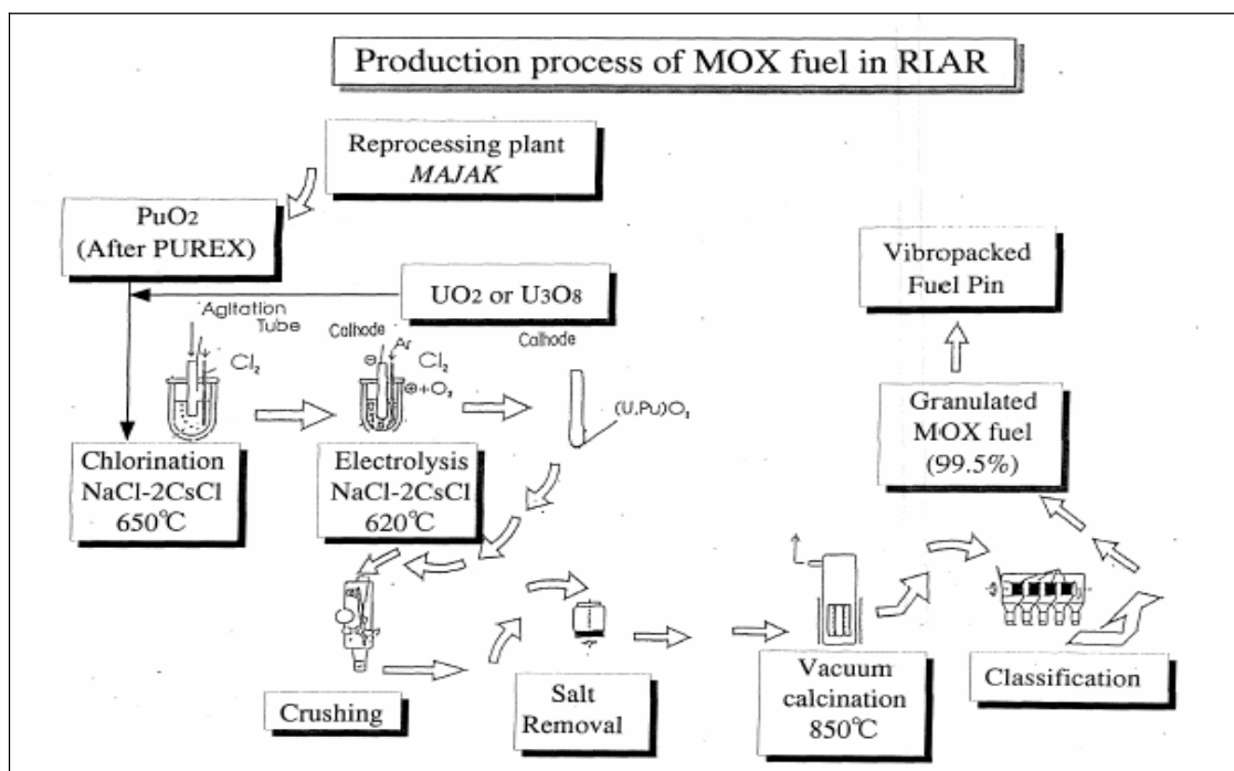
Figure D1-15. The VIPAC process and its relation to pyrochemical reprocessing technology.
