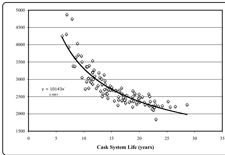
Figure O-7. Variation of the daily rental rate for cask system reusable components with component useful life.
