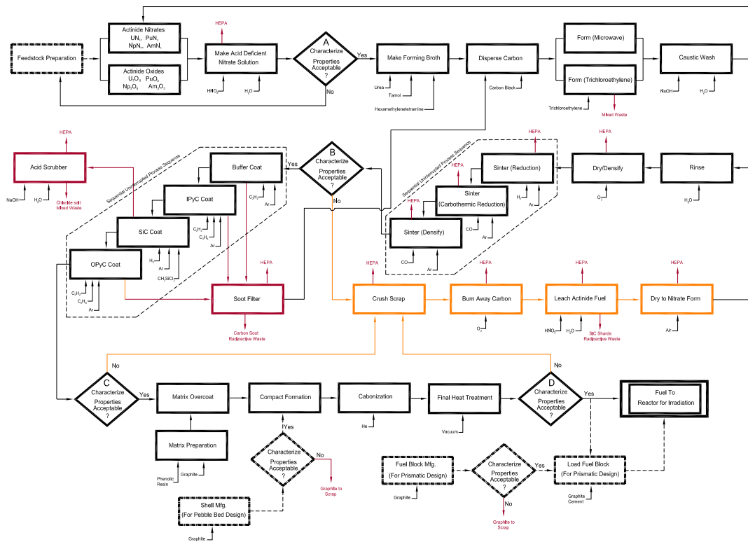
TRISO MOX Fuel Process Flow Diagram
