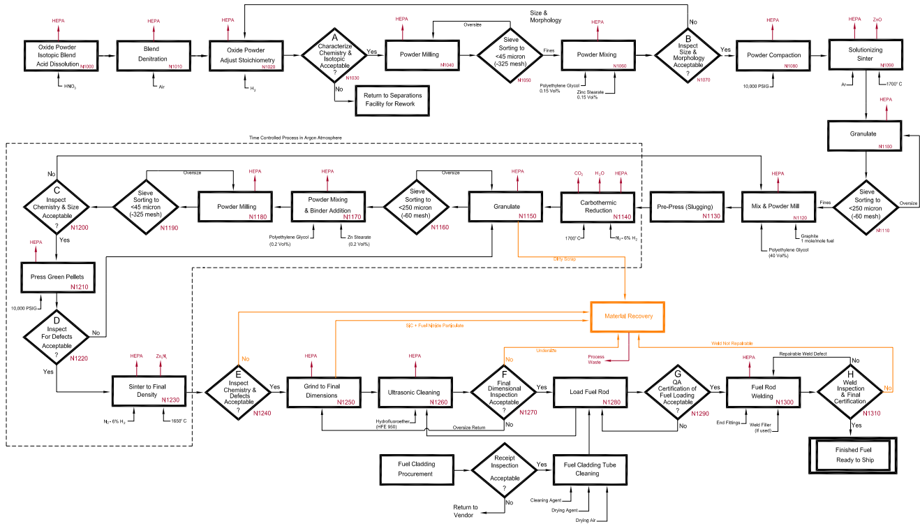
Figure D1-12. Fabrication process for mixed nitride fuels.
